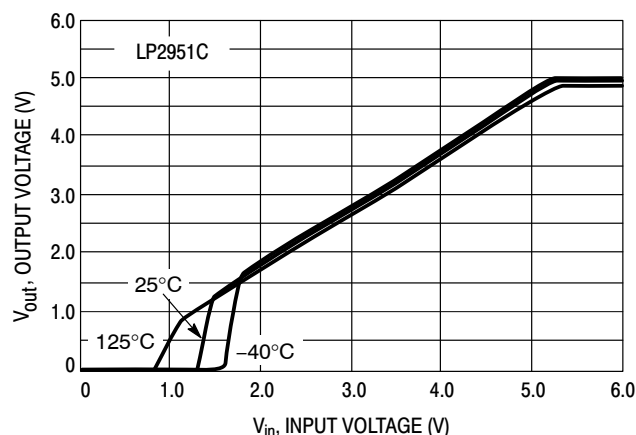
Figure 5. 5.0 V Dropout Characteristics with R_L = 50 \text{ }\Omega
