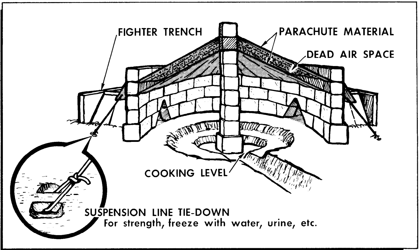
Figure 15-19. Para-Snow House.
