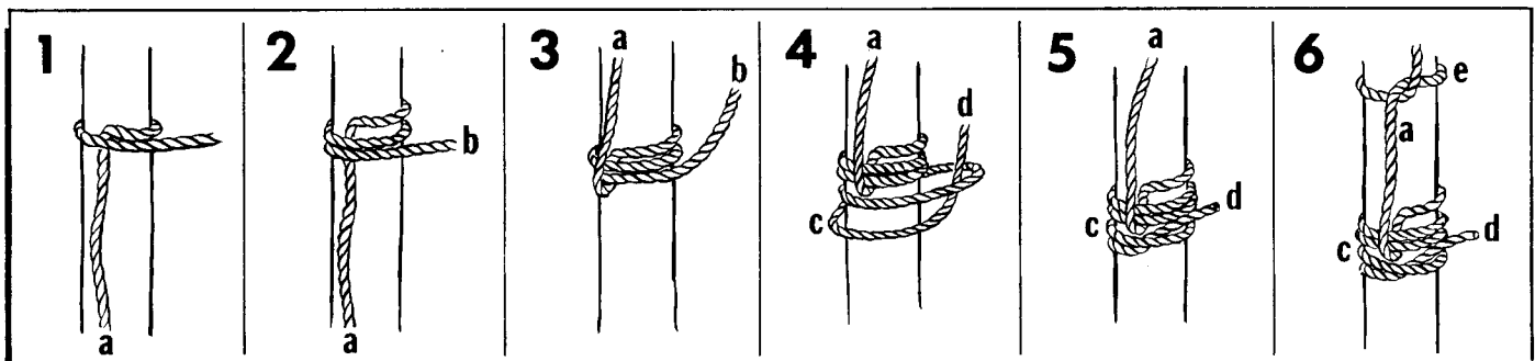
Figure 17-52. Rolling Hitch.
