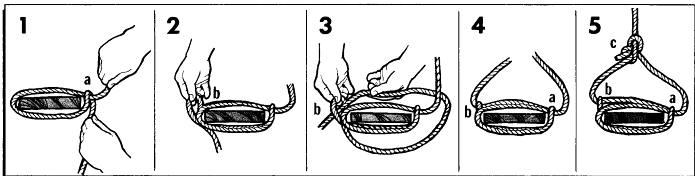
Figure 17-55. Scaffold Hitch.
