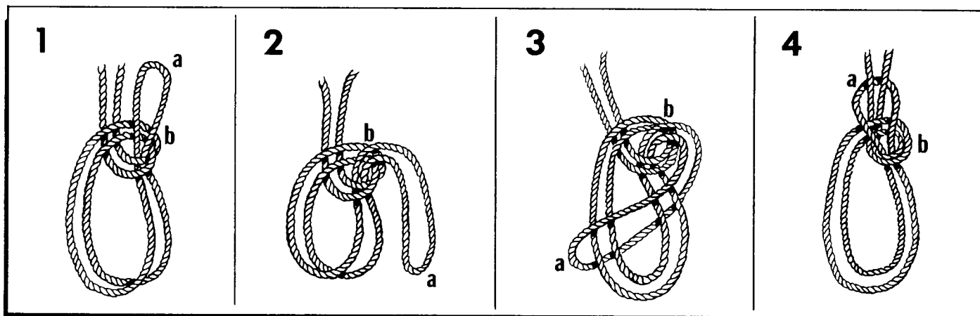
Figure 17-43. Bowline on a Bight.
