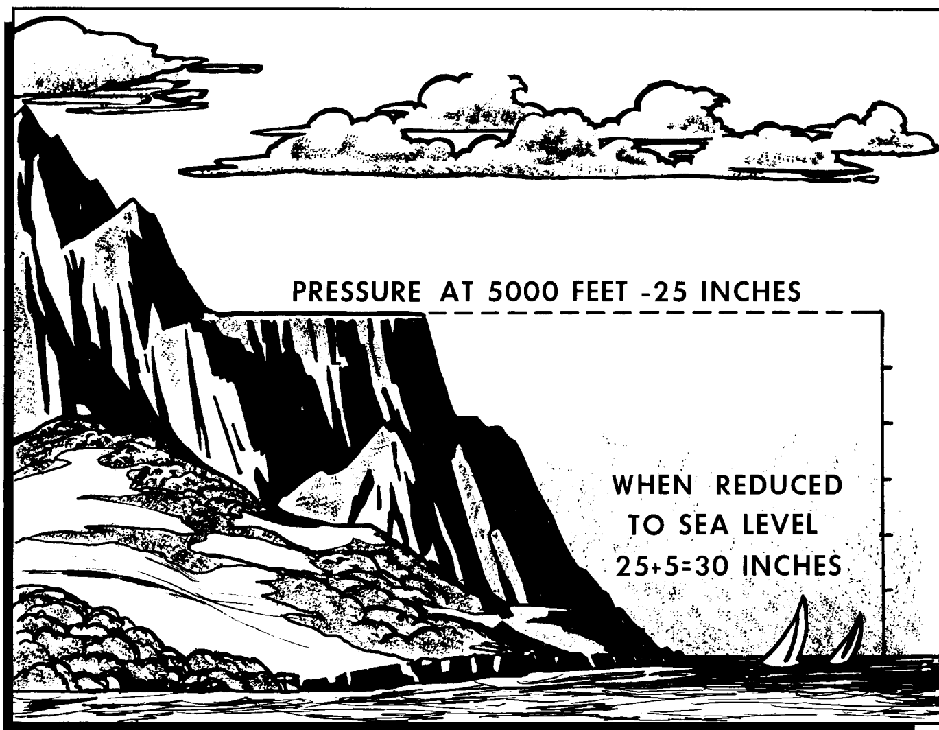
Figure 9-2. Air Pressure.
