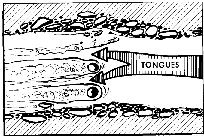
Figure 23-26. Tongue of the Rapids.
