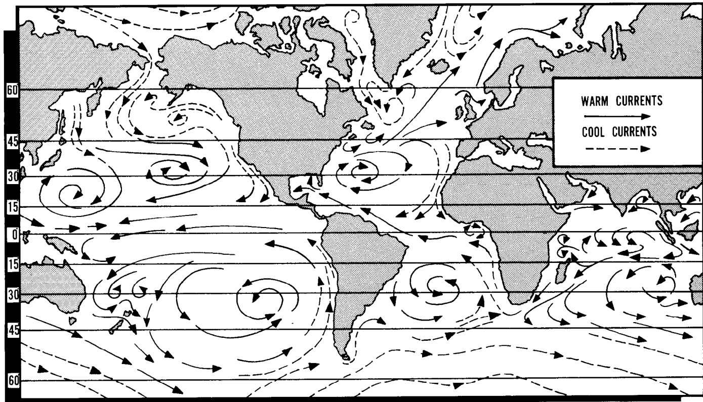
Figure 11-39. Ocean Currents.
