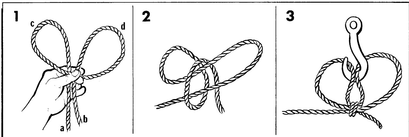
Figure 17-54. Catspaw.
