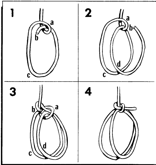
Figure 17-45. French Bowline.
