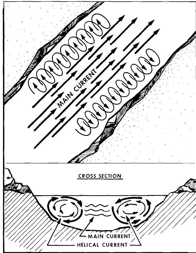
Figure 23-13. Helical Flow.
