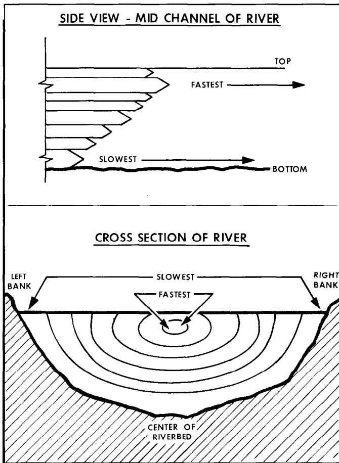
Figure 23-12. Laminar Flow.
