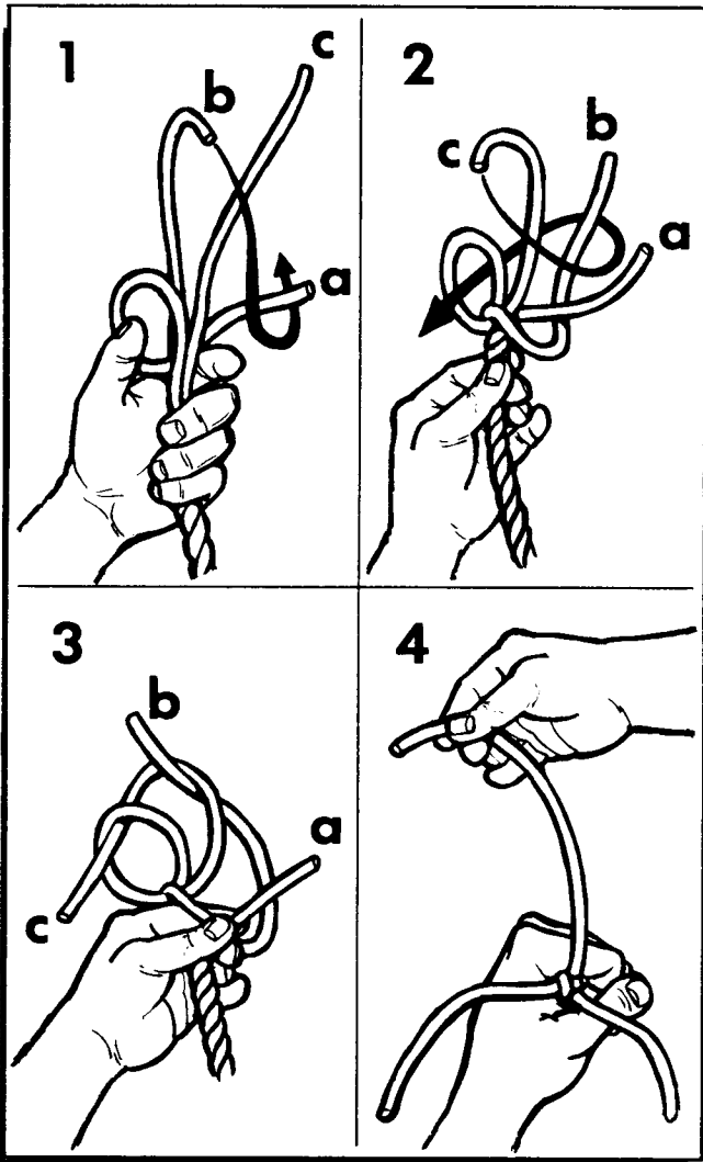
Figure 17-31. Wall Knot.
