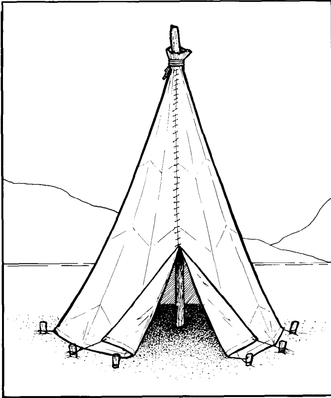
Figure 15-6. 1-Pole Tepee.
