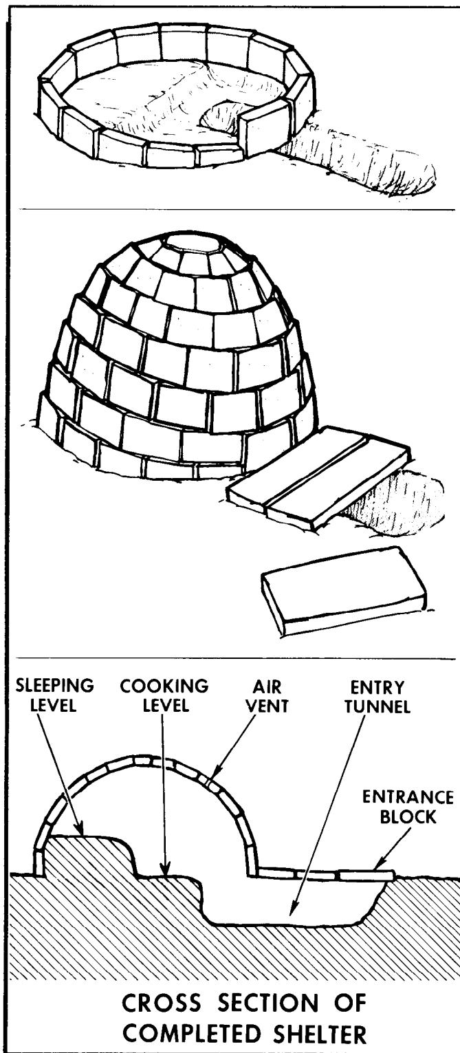
Figure 15-18. Igloo.
