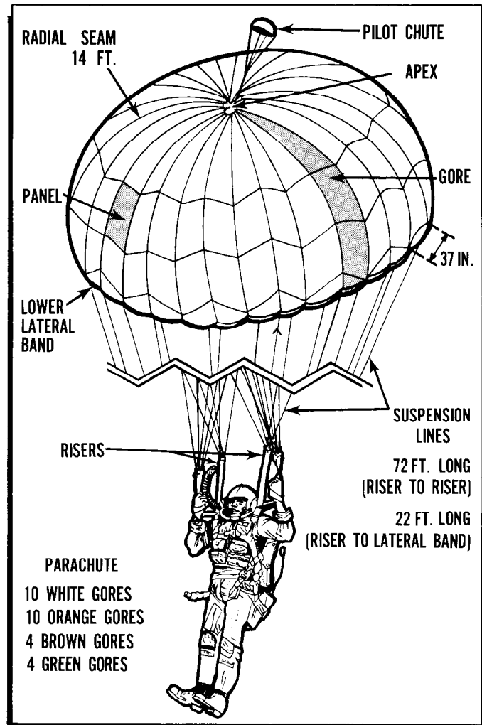
Figure 17-16. Parachute Diagram.
