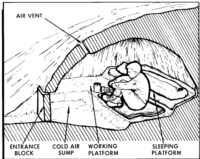
Figure 15-27. Snow Cave Shelter Living.
