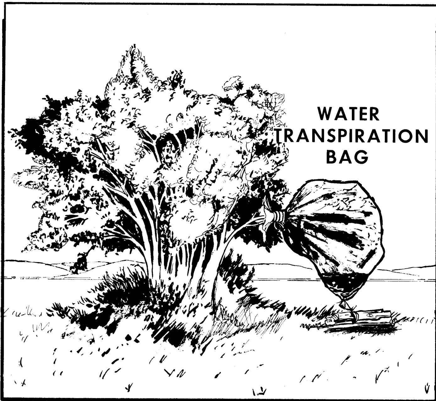
Figure 19-13. Transpiration Bag.
