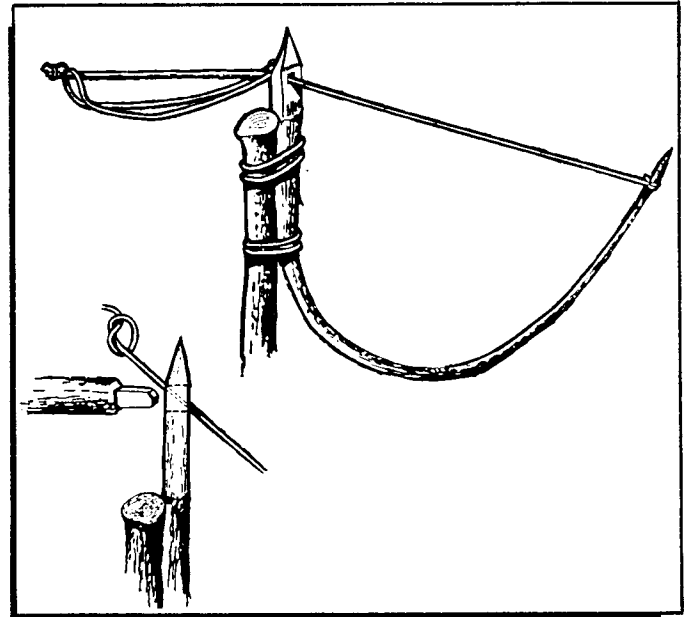
Figure 18-16. Ojibwa Bird Snare.
