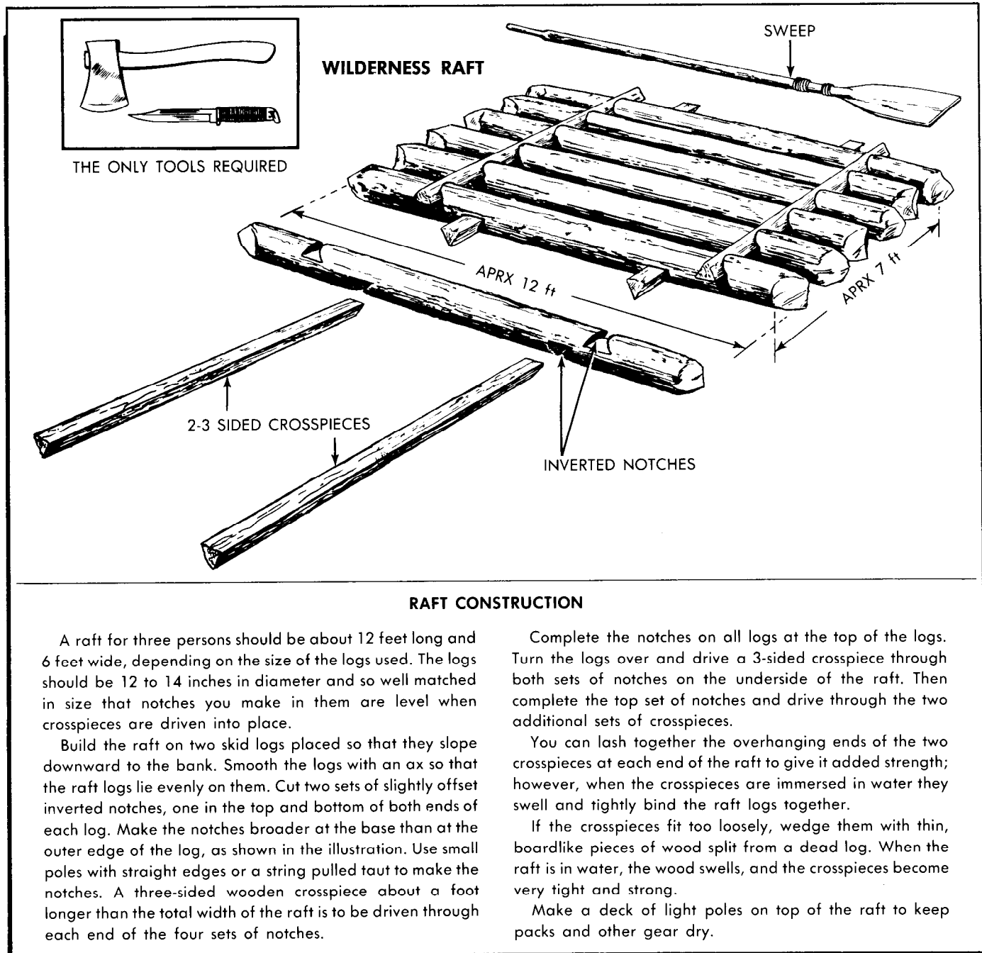
Figure 23-36. Raft Construction.
