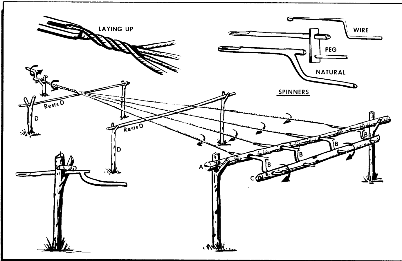
Figure 17-62. Rope Machine.
