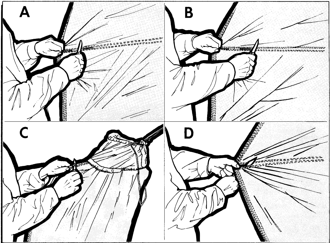
Figure 17-17. Cutting the Parachute.
