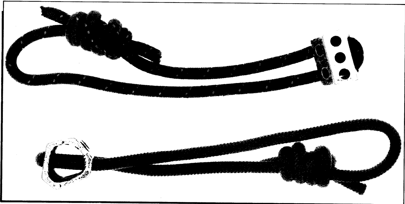
Figure 22-21. Hexcentric Chock with Kernmantle Sling.
