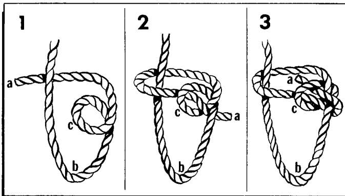
Figure 17-42. Running Bowline.
