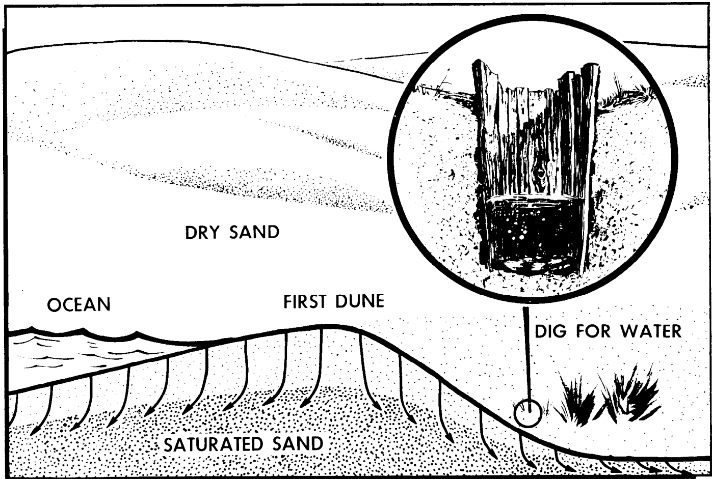
Figure 19-3. Beach Well.
