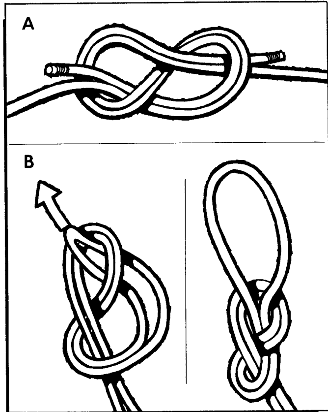
Figure 22-6. Figure-Eight Loop.
