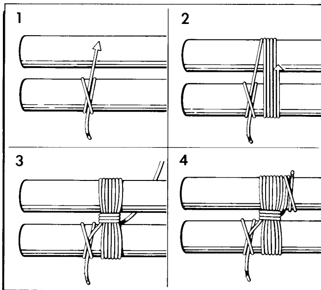
Figure 17-60. Shear Lash.
