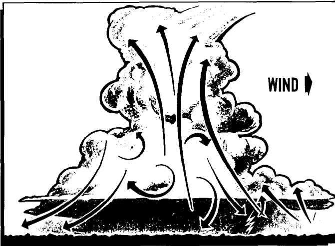
Figure 9-12. Thunderstorms.
