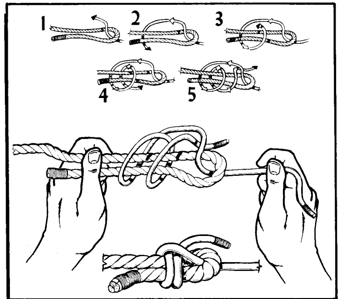
Figure 17-36. Double Sheet Bend.
