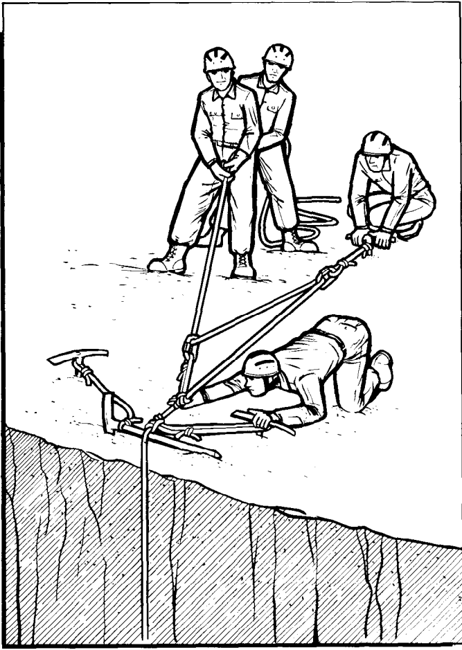
Figure 22-96. Two-Pulley System.
