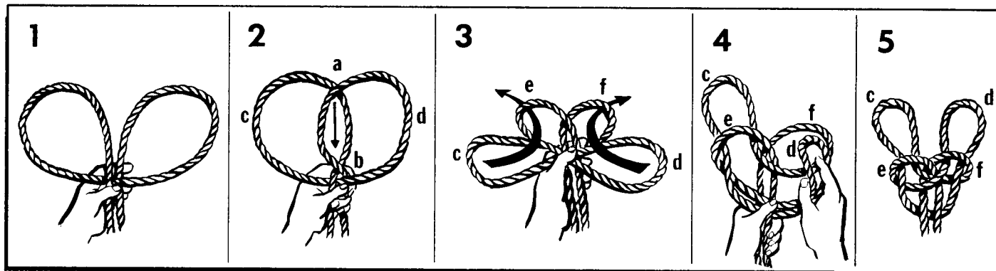
Figure 17-44. Spanish Bowline.
