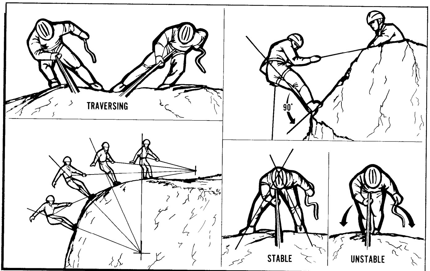
Figure 22-54. Body Position for Rappel.
