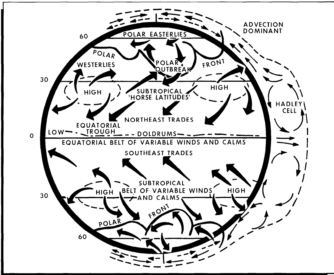
Figure 9-7. Atmosphere Circulation.
