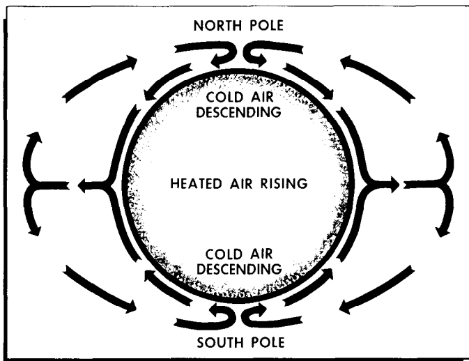
Figure 9-3. Wind Movement.
