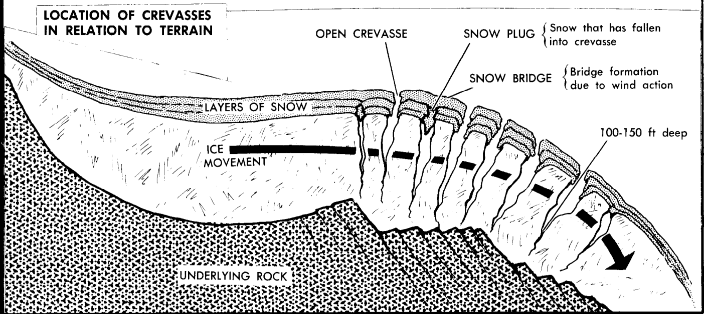
Figure 22-68. Typical Glacier Construction.
