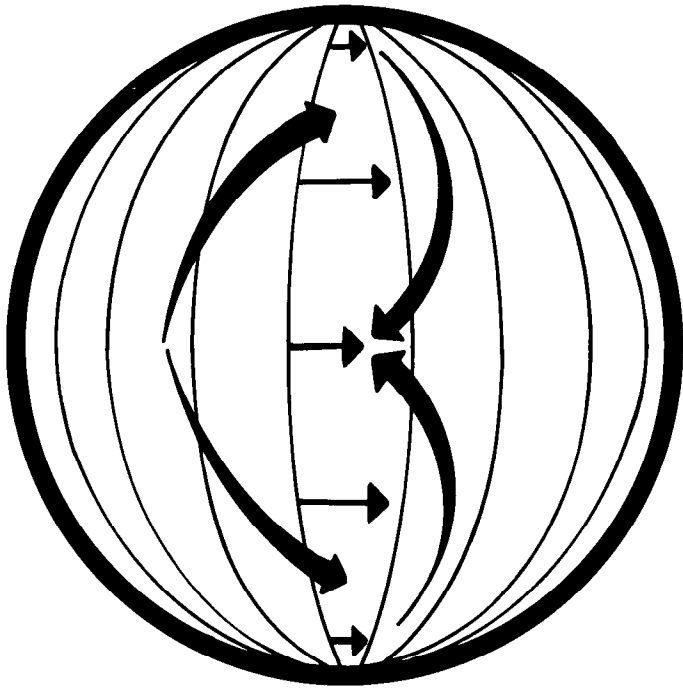
Figure 9-6. Coriolis Effect.
