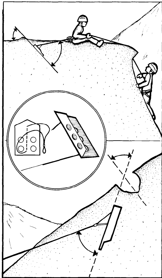
Figure 22-61. Snow Flukes.
