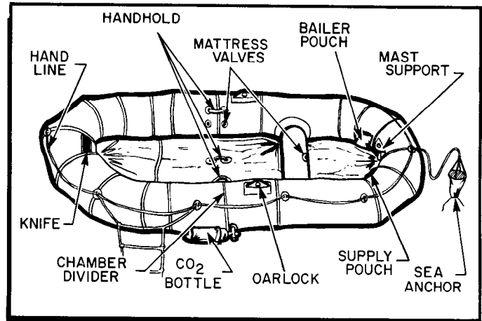
Figure 23-48. Seven-Man Raft.
