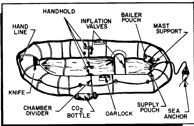
Figure 23-3. Seven-Man Raft.
