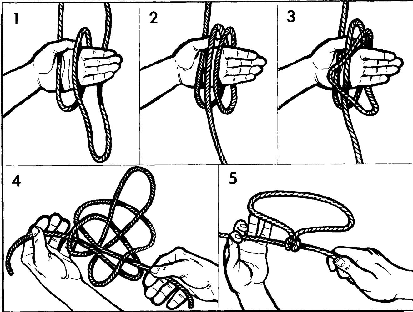
Figure 22-8. Butterfly Knot.
