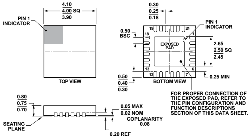
Figure 75. 24-Lead Lead Frame Chip Scale Package [LFSCP_WQ] 4 mm × 4 mm, Very Very Thin Quad (CP-24-7) Dimensions shown in millimeters
