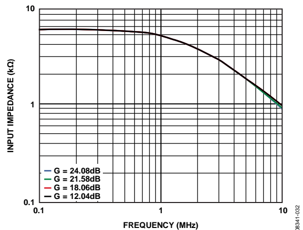
Figure 13. Input Impedance R_{IN} vs. Frequency, Untermated
