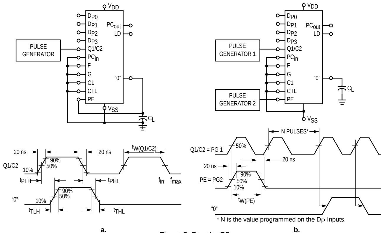
Figure 3. Counter D2
