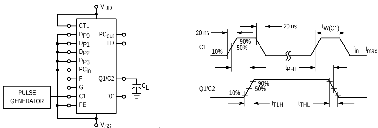
Figure 2. Counter D1
