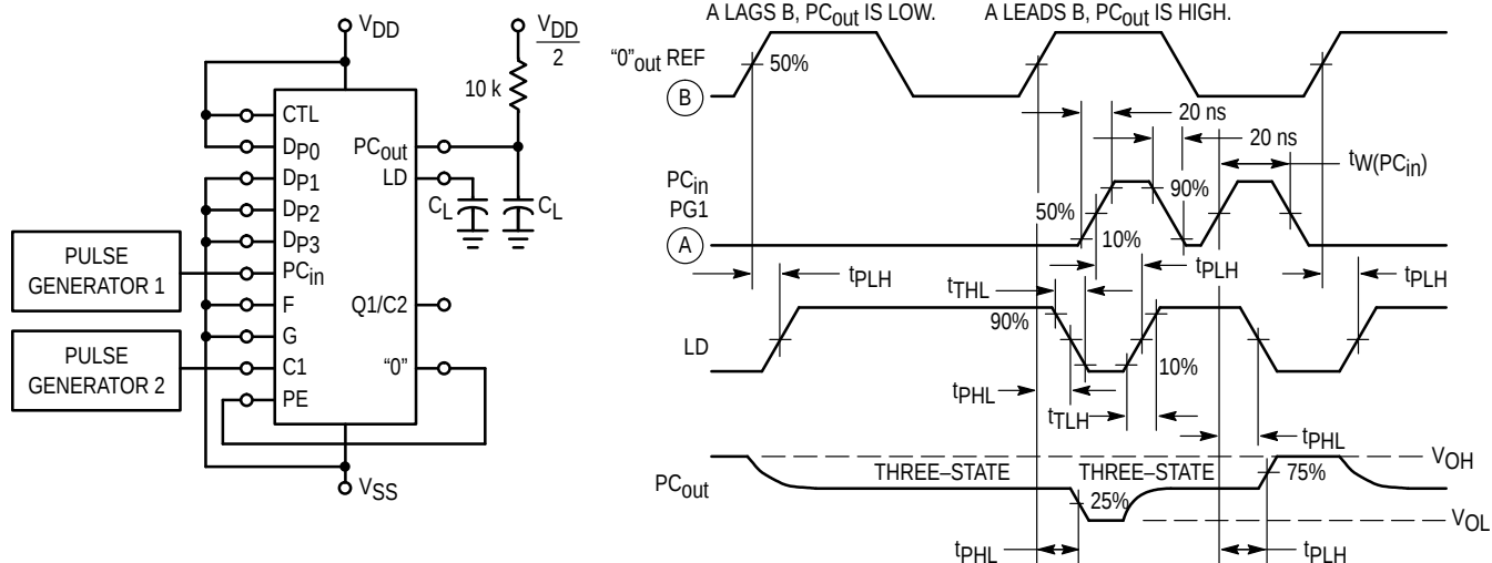
Figure 1. Phase Comparator
