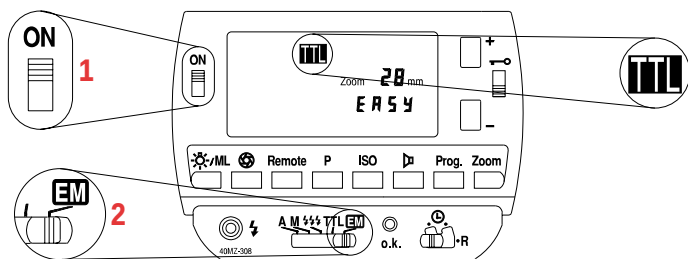
Fig. 8: Settings for TTL Easy Mode
