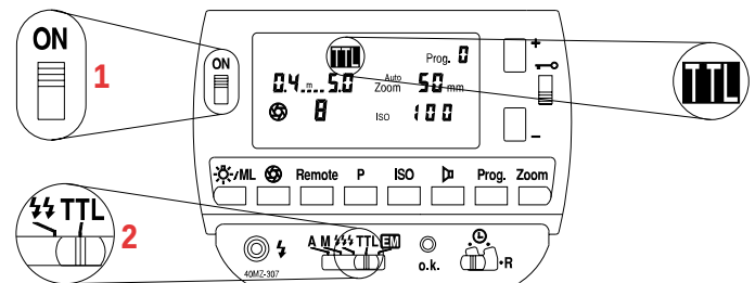
Fig. 7: Settings for TTL mode
