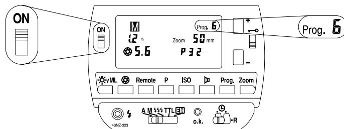
Fig. 23: Display of an activated user program
