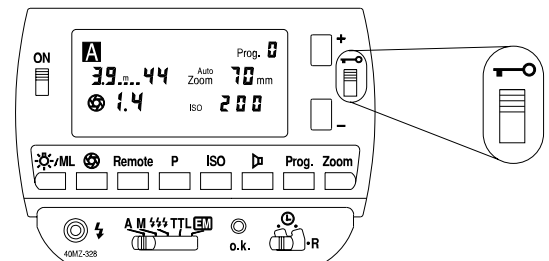
Fig. 29: Locking the controls
