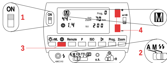
Fig. 12: Settings for manual mode
